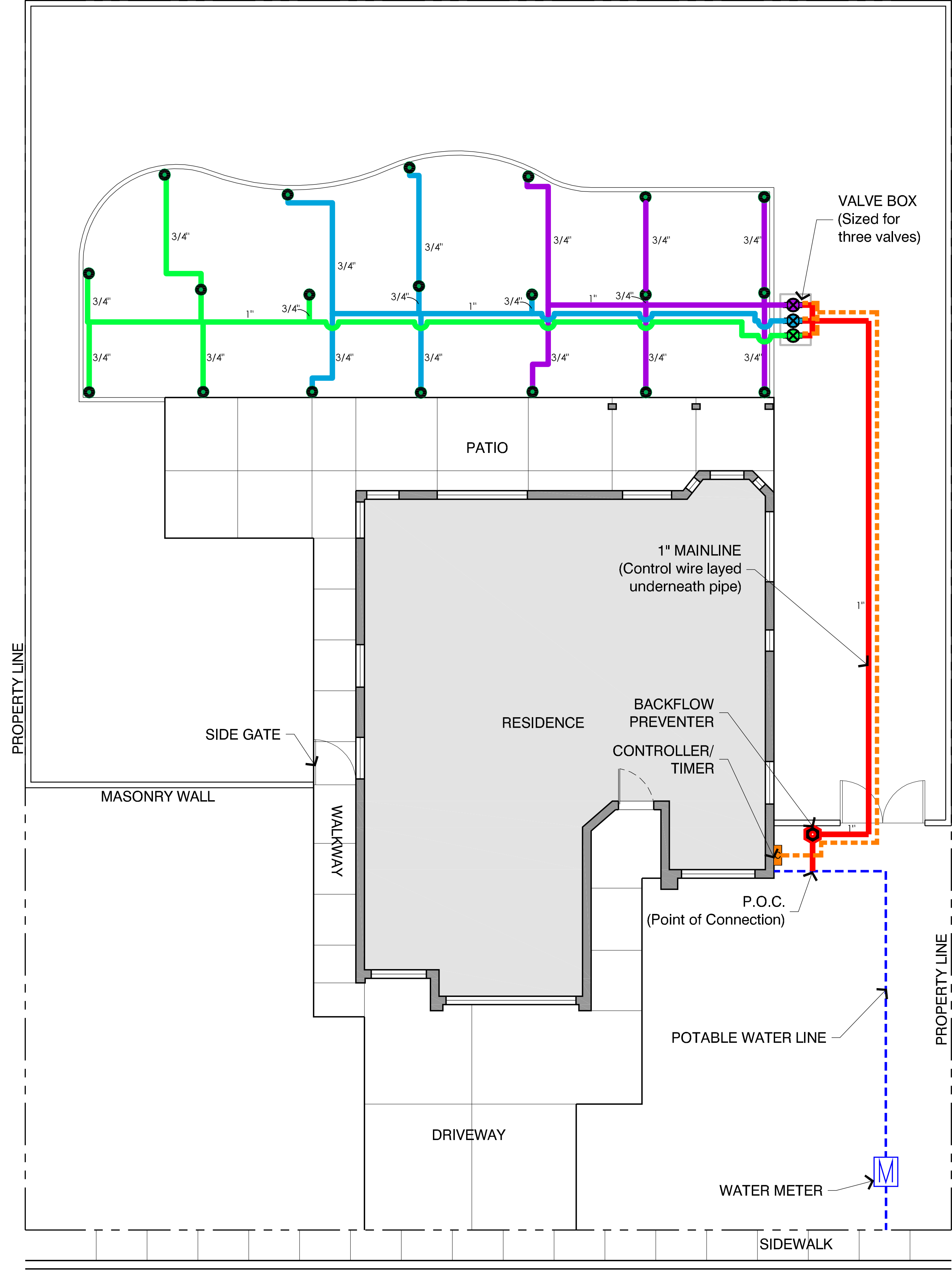
2 PIPE LAYOUT
