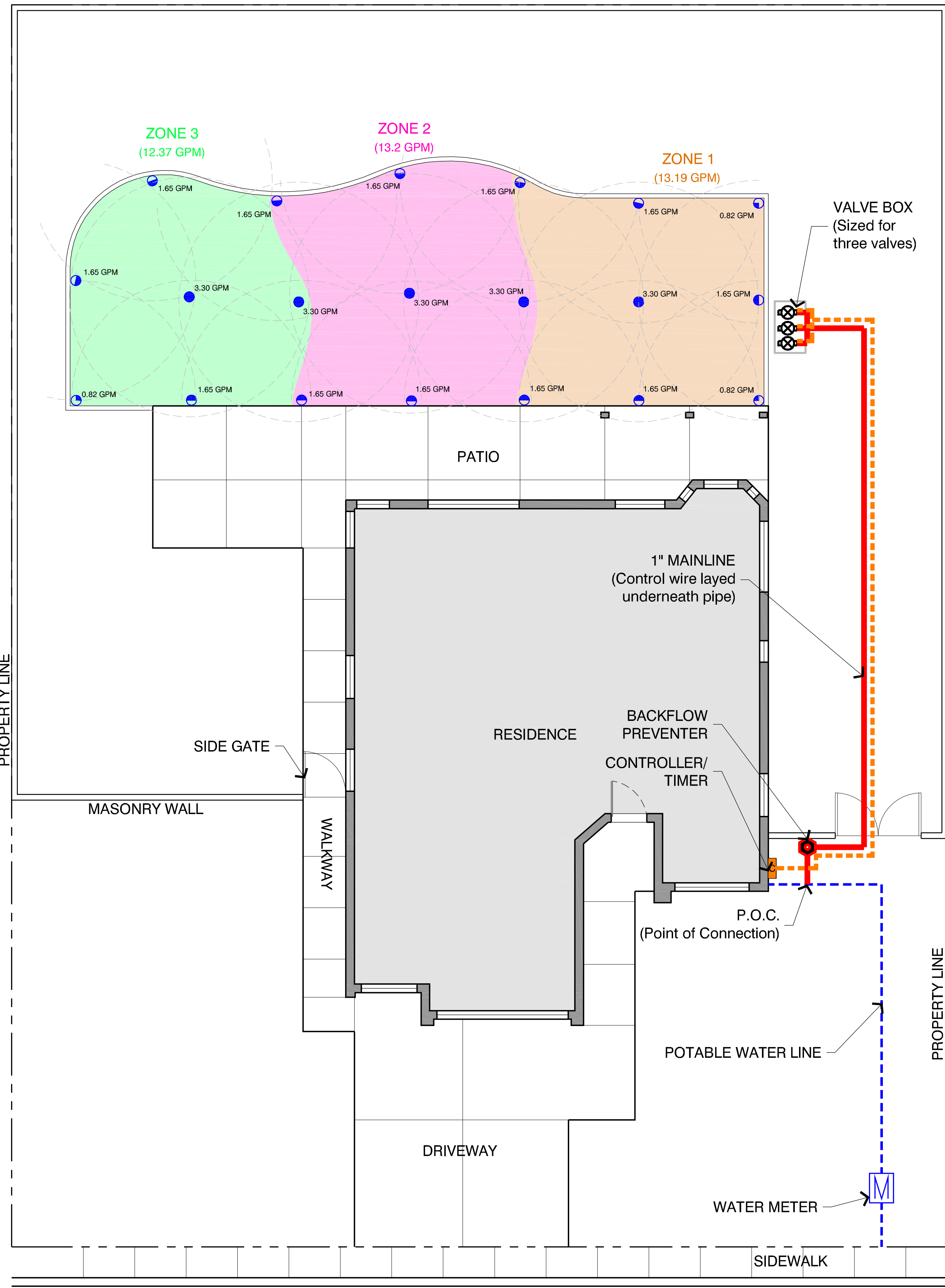
1 SPRINKLER LAYOUT
